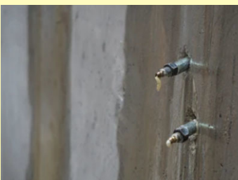
4) Injection grouting
